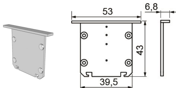
550-585-xx Embout de finition Epic WING
