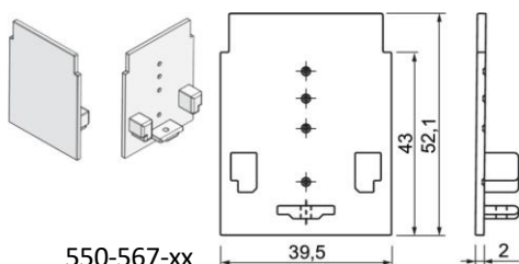
550-567-xx Embouts de finition Epic III
